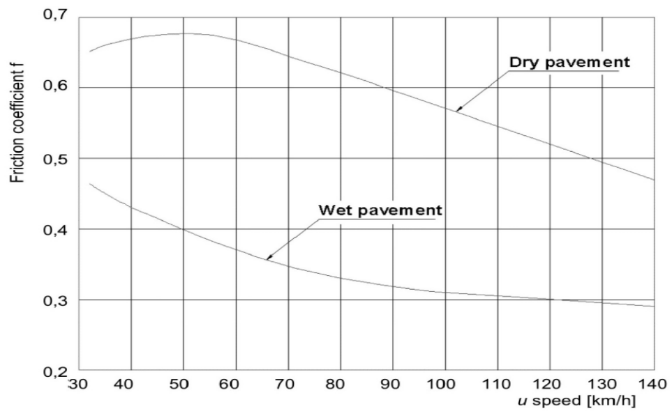
Figure S2. Determination of the coefficient of friction between the tire and the road. 9
