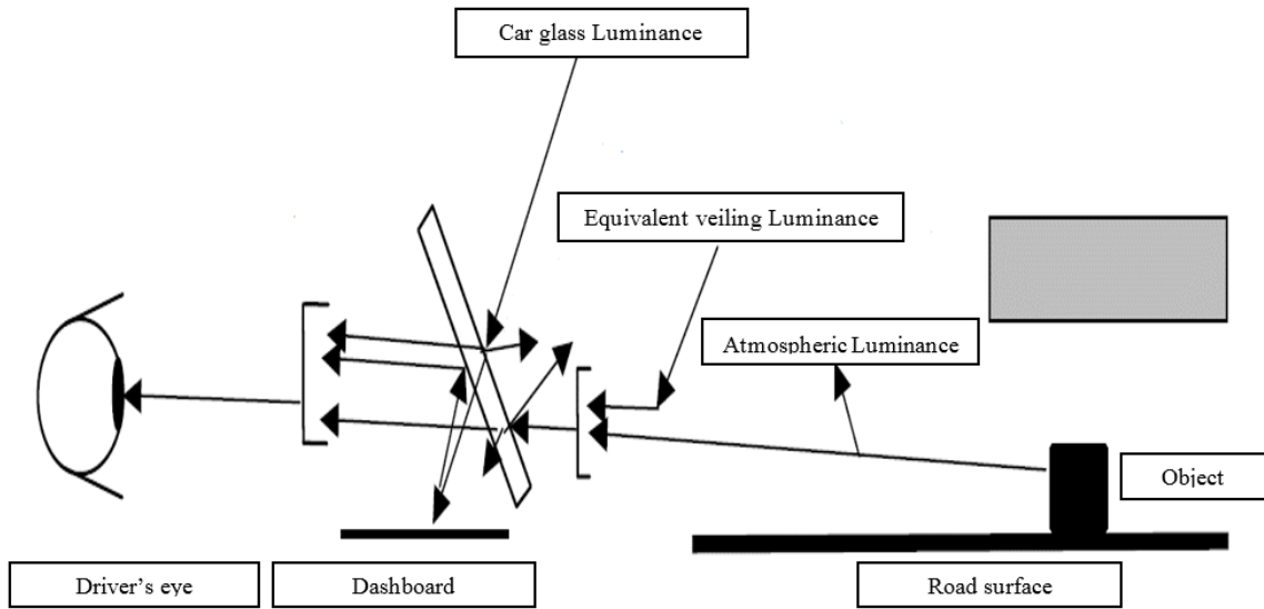
Figure S1. Factors affecting the disability glare at the entrance of tunnels. 9
